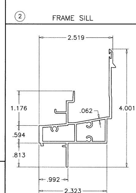
②A FRAME SILL (INTERMEDIATE)
