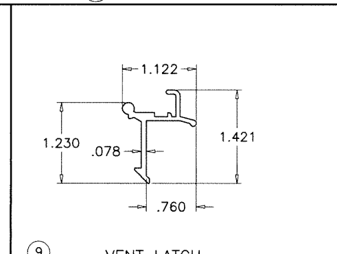
⑨ VENT LATCH
