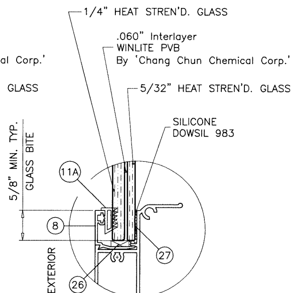
GLASS TYPE 'DR'
