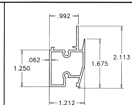
④ MEETING RAIL FOR SPRING LATCH
