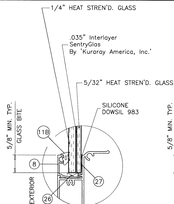
GLASS TYPE 'BR'
