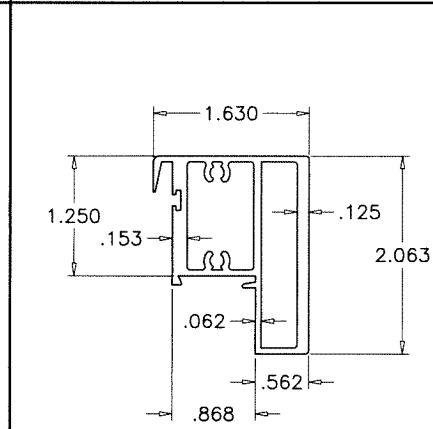
⑤A VENT TOP RAIL FOR SWEEP LATCH
