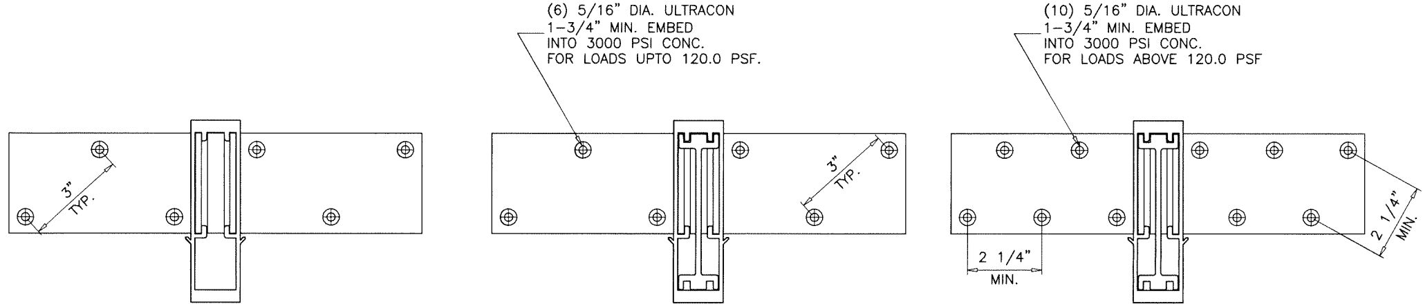
MULLION WITHOUT REINF.
