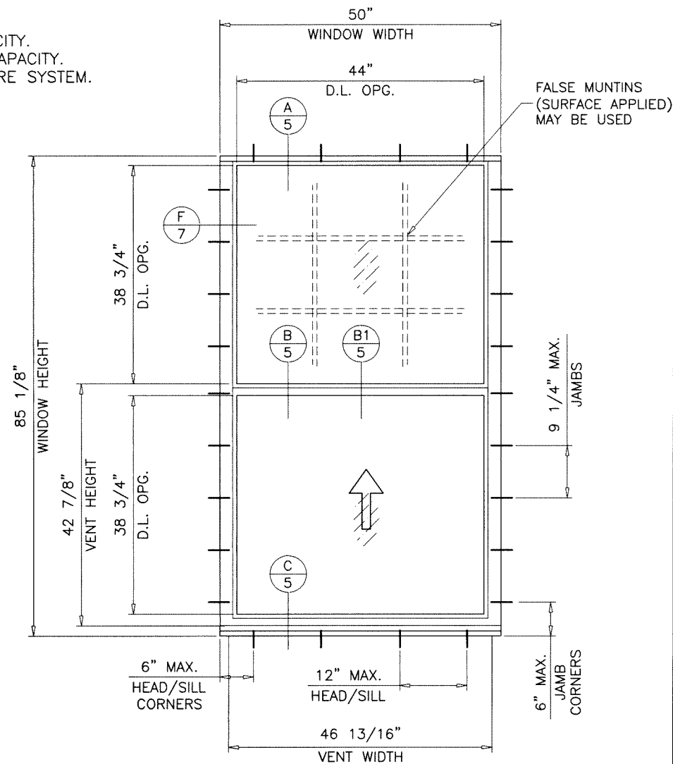
TYPICAL ELEVATION
