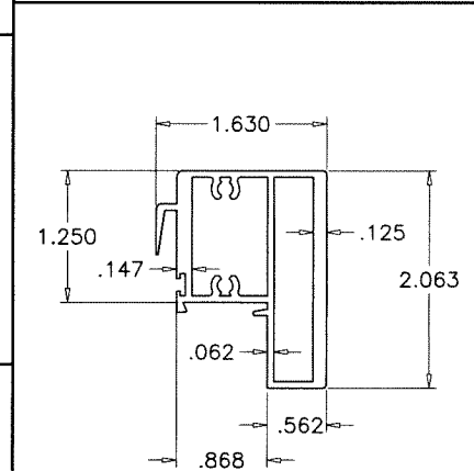
⑤ VENT TOP RAIL FOR SPRING LATCH
