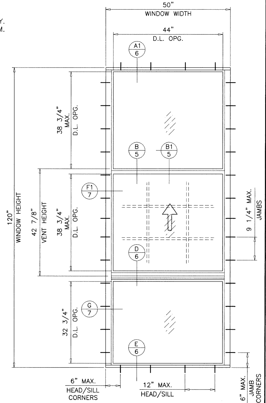
TYPICAL ELEVATION
